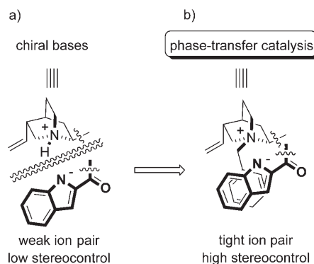
Figure 1. Chiral organic bases versus phase-transfer catalysis in the enantioselective ring closure of 3 .
