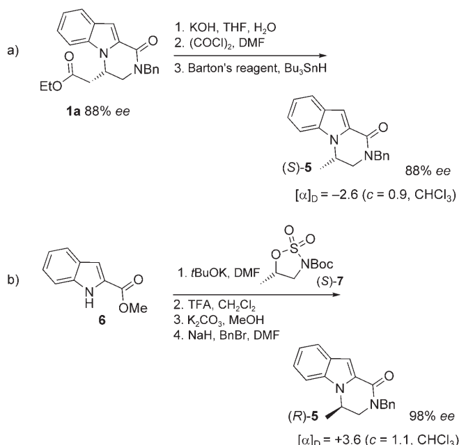
Scheme 3. Determination of the absolute configuration of product 1a . THF: tetrahydrofuran; DMF: N,N -dimethylformamide; Boc: tert -butoxycarbonyl; TFA: trifluoroacetic acid.
