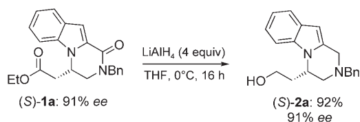
Scheme 4. Stereoretentive synthesis of pyrazino-indole 2a from pyrazino-indol-1-one 1a .
