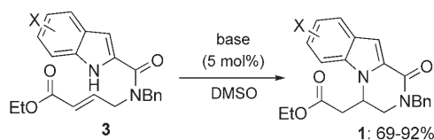
Scheme 2. Base-catalyzed synthesis of 1 . Bn: benzyl; DMSO: dimethylsulfoxide.
